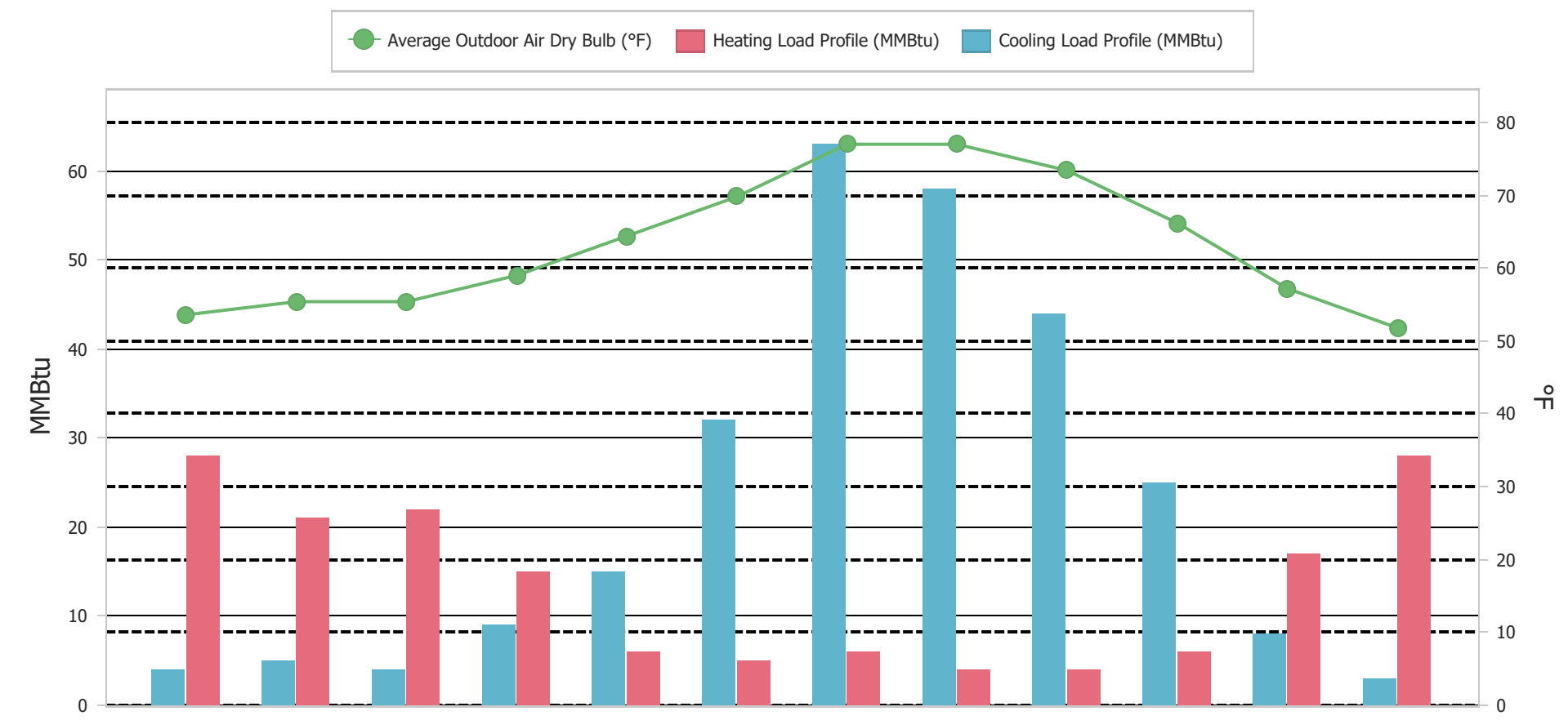
Site HVAC Load Profile
